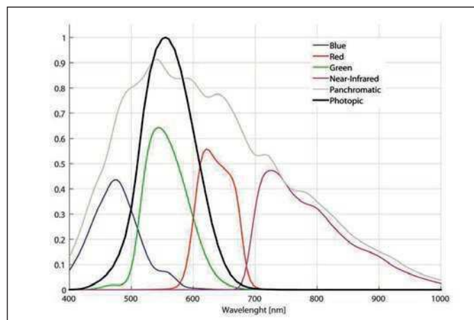
▲ Figure 2, The photopic curve (black line) together with the spectral sensitivity of DMC bands.
