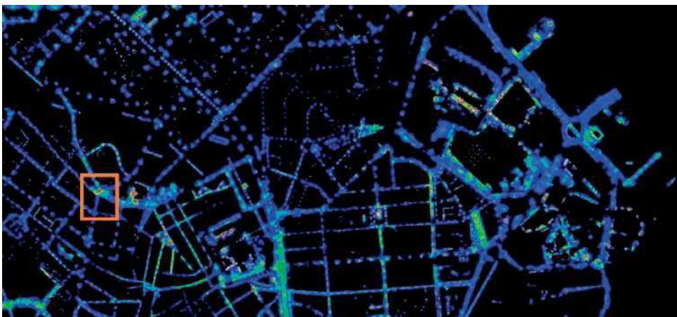
▲ Figure 4, Luminance map obtained from fusing VNIR and DMC data, GSD 1m. Legend as in Figure 3.
