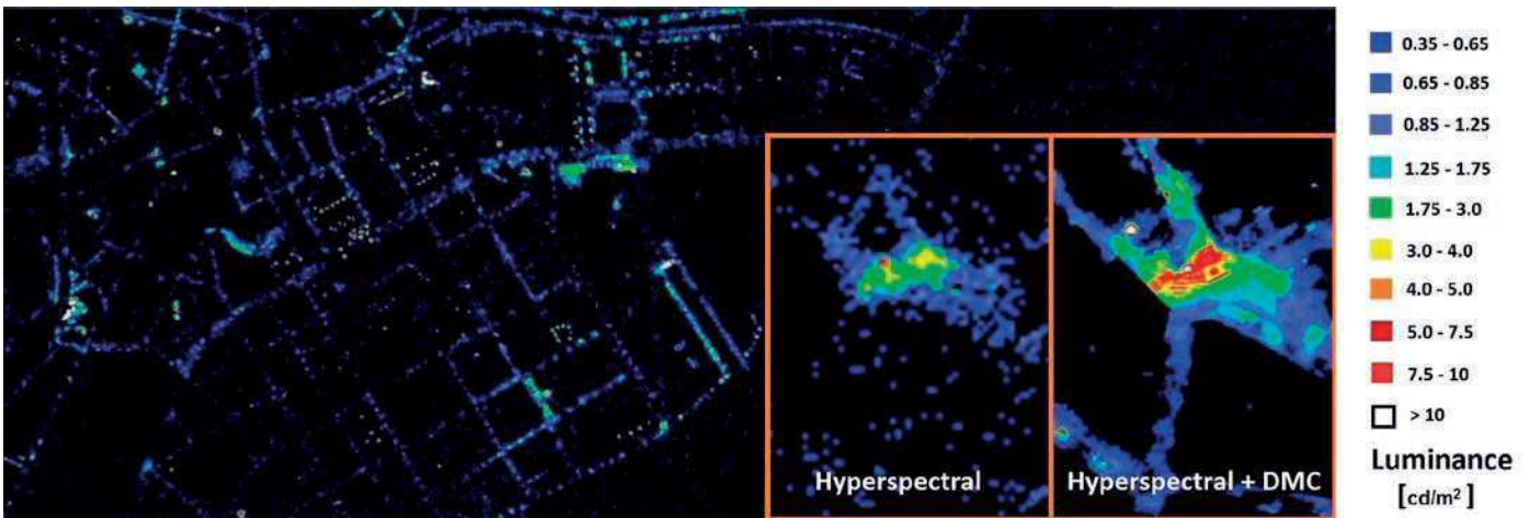
▲ Figure 3, VNIR luminance map obtained from hyperspectral VNIR imagery, GSD 1.5m. Pixels with a luminance <0.35cd/m 2 are black. The two insets cover the area outlined in orange in Figure 4.
