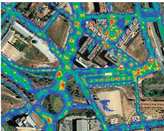
▲ Figure 5, Detail of the final luminance map, GSD 0.25m. For pixels with a luminance <0.35cd/m 2 the underlying orthoimage is shown. Legend as in Figure 3.
